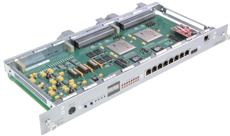
Figure 2: The Cadence SpeedBridge Adapter for Ethernet
