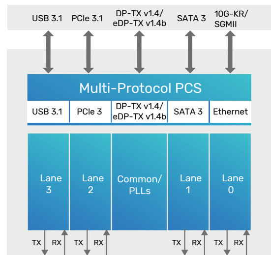
Figure 1: Example system-level block diagram
