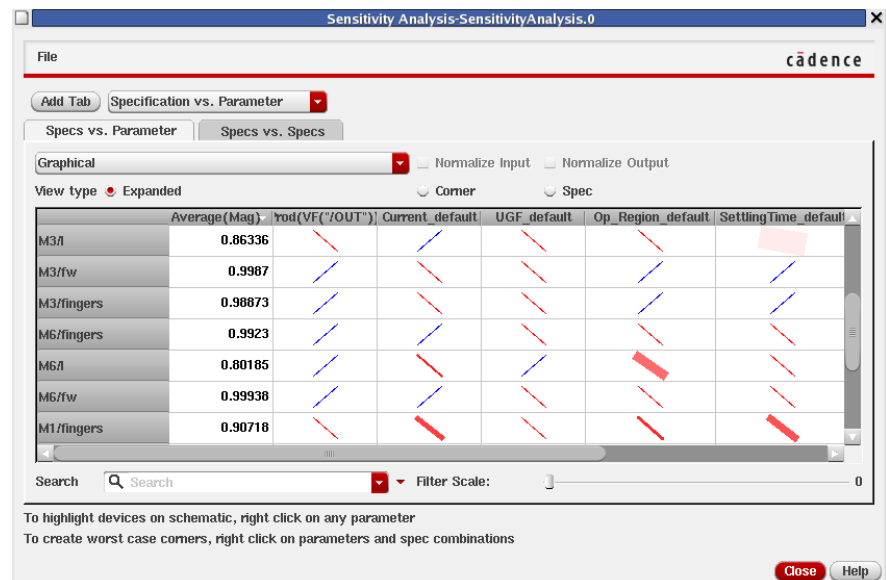
Figure 4: Sensitivity of device parameters to measured goals
