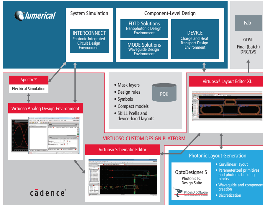
Figure 4: Electronic/photonic design automation (EPDA) environment
