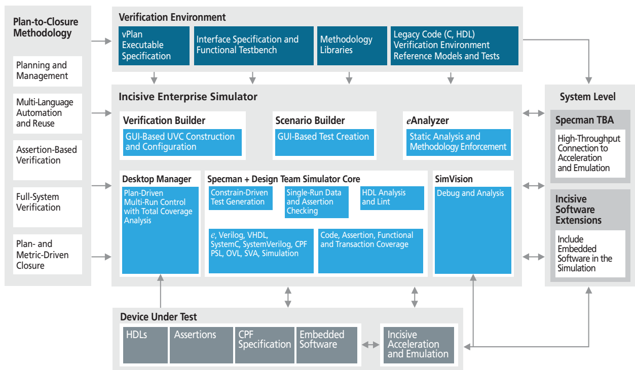
Figure 1: Incisive Enterprise Specman Elite® Testbench helps drive the entire process of verification at block, chip, system, and project levels. The Verification Builder, Scenario Builder, and eAnalyzer components automate the creation and configuration of reusable, scalable, eRM-compliant environments and stimuli. Incisive Software Extensions offer a high-throughput channel between the testbench and the device under test (DUT), and enable access to embedded software as if it were another part of the DUT.
