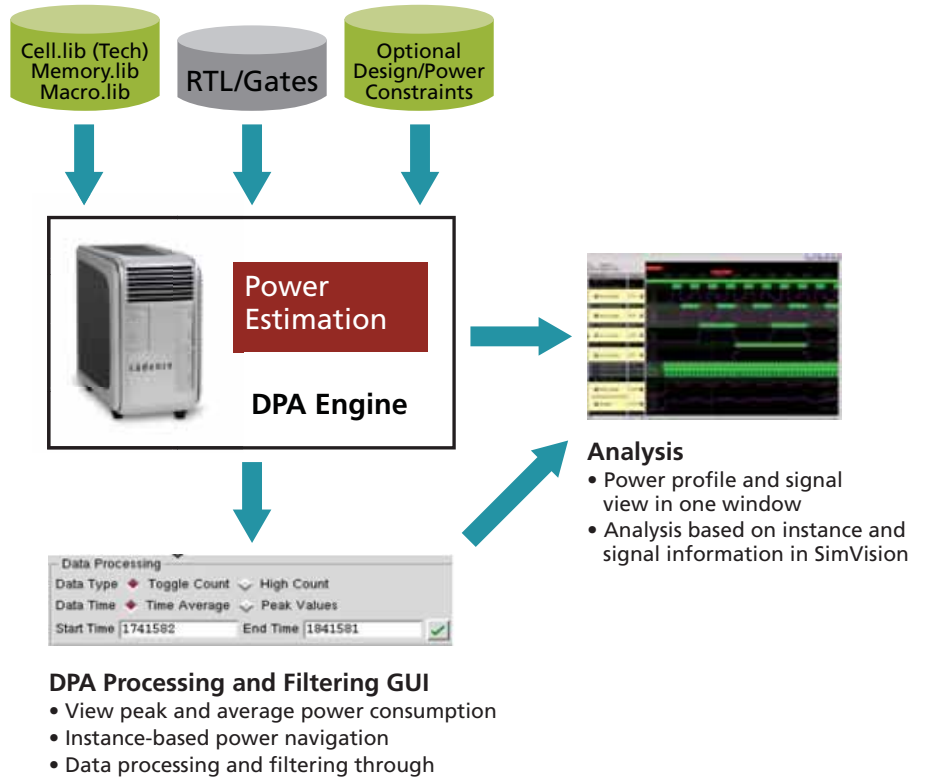
Figure1: Palladium Dynamic Power Analysis user flow
