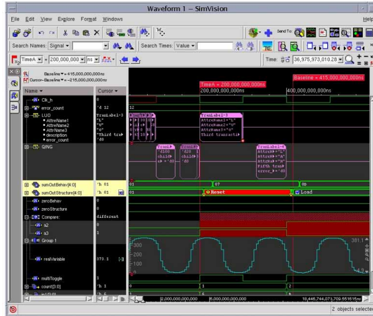
Figure 3: The SimVision integrated debug environment supports signal-level and transaction-based flows across all IEEE-standard design, testbench, and assertion languages, in addition to concurrent visualization of hardware, software, and analog domains.
