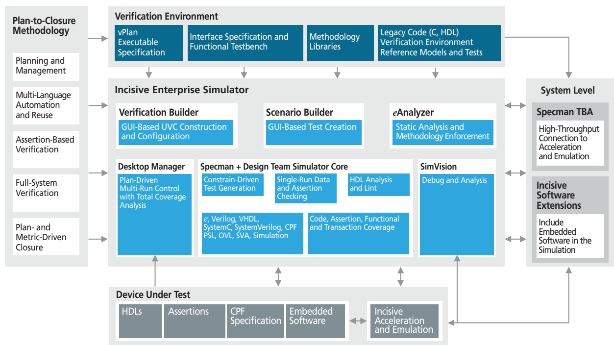
Figure 1: Incisive Enterprise Simulator combines Incisive Enterprise Specman ® Simulator, SimVision, Desktop Manager, Verification Builder, Scenario Builder, eAnalyzer, and the Plan-to-Closure Methodology in a single optimized package. Engineers can “hot-swap” the state of the software-based simulation in and out of the Incisive Xtreme ® series of accelerators and emulators for additional performance. System-level capabilities include a connection to Incisive Software Extensions and support for testbench acceleration with Palladium ® XP.
