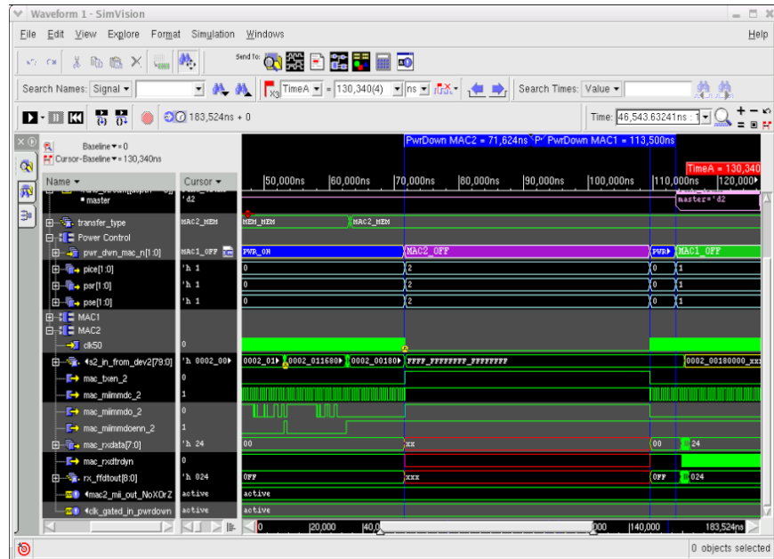
Figure 4: Engineers can determine the DUT’s power characteristics very early in the project life cycle. In this example, the user is verifying a full cycle of power shut off (note the Xs in the center) and correct state restoration.
