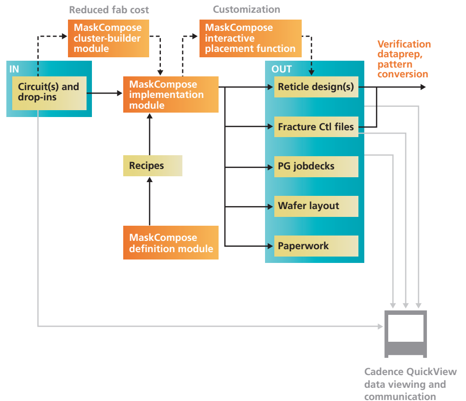
Figure 1: MaskCompose schematic overview
