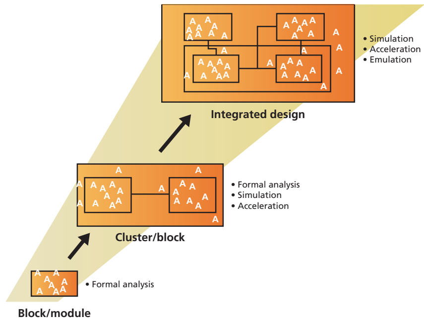
Figure 2: Formal analysis at the entry point of the Incise platform's complete assertion-based verification flow
