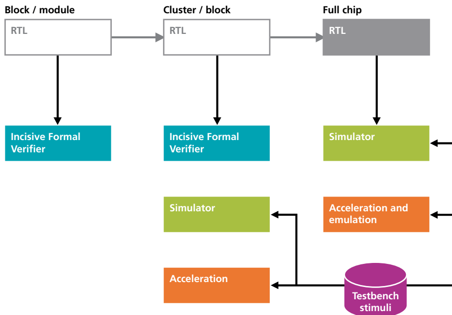
Figure 1: Incisive Formal Verifier brings formal analysis to the designer's desktop
