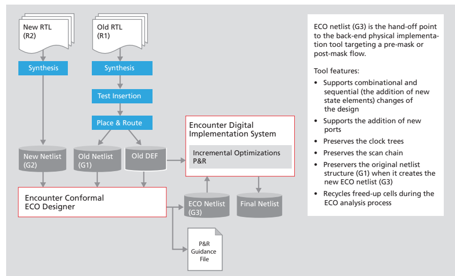
Figure 2: The Encounter Conformal ECO Designer implementation flow
