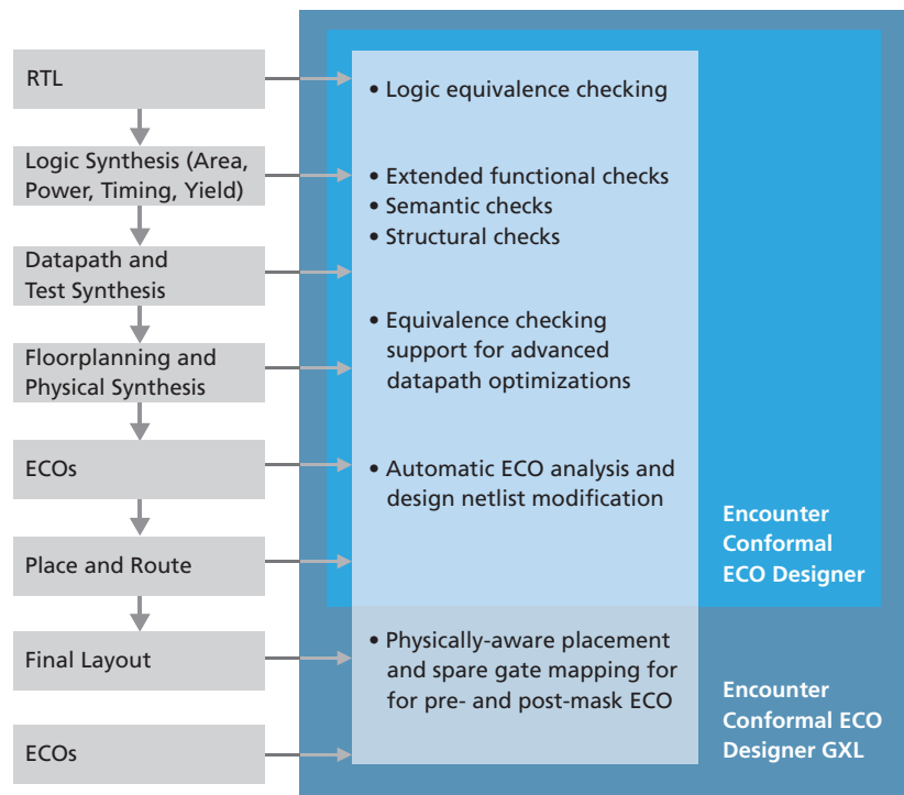
Figure 1: Encounter Conformal ECO Designer offers automatic ECO analysis and design netlist modification
