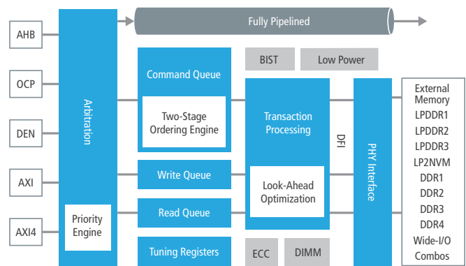
Figure 1: Cadence Design IP for DDR DRAM delivers the lowest-risk path to the highest-performance, lowest-power designs
