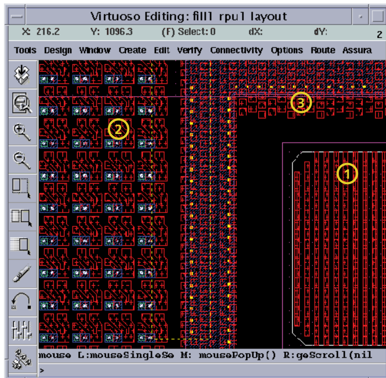
Figure 2. Sample context-dependent fill recipe: rectangular fill (1) under bond pad, grounded multi-layer custom fill (2) pattern in empty areas, skewed square fill (3) under power lines.
