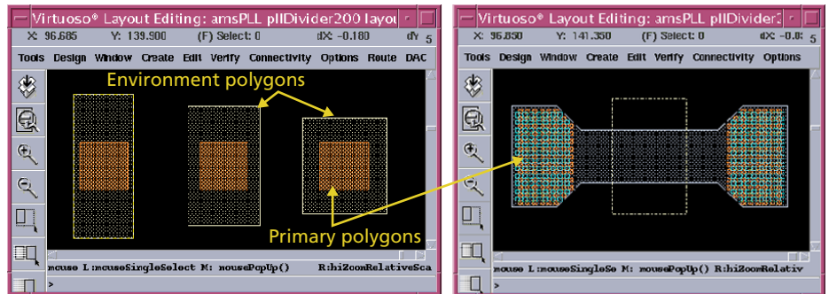
Figure 1: A set of design rules are described by drawings in a model file (GDSII, DFII, text vertices). A model contains a primary polygon (e.g., contact, fuse opening, DRC error markers) and environment polygons (e.g., metals enclosing contact, fuse metals/vias, waivable layout configuration per error marker). Pattern check is triggered by primary polygons in the design.
