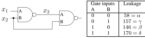
Figure 1: Example circuit for leakage minimization and leakage power values dissipated in both NAND gates as a function of their inputs.
