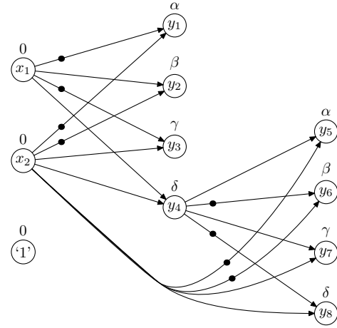
Figure 2: AND/INVERTER graph for circuit from Figure 1. Nodes represent the inputs x_1 , x_2 , the constant '1', and AND gates. Labels above each node are weights representing leakage.
