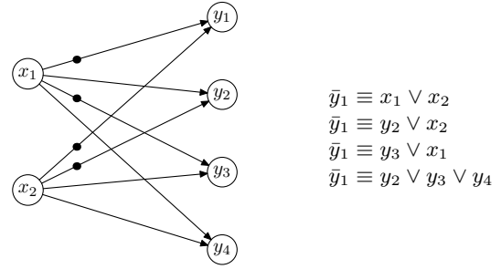
Figure 3: Valid facts about \bar{y}_1 .
