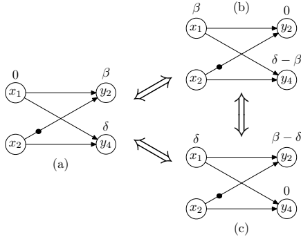
Figure 4: Valid moves preserve the objective.
